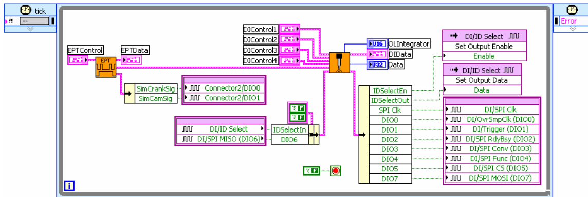
Figure 17. LabVIEW FPGA Block diagram example.
