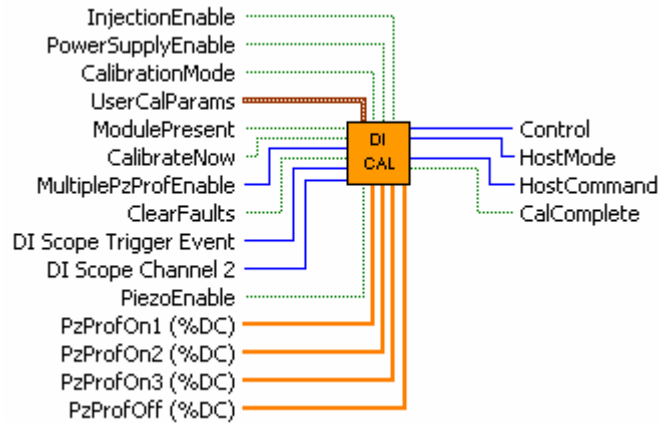
Figure 15. di_vt_rt_cal_revx.vi VI icon with leads.
