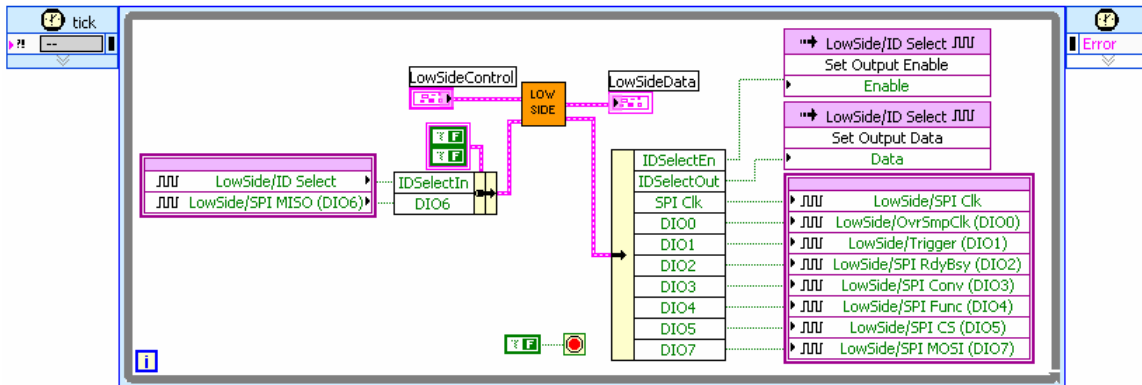
Figure 9. LabVIEW FPGA Block diagram example.
